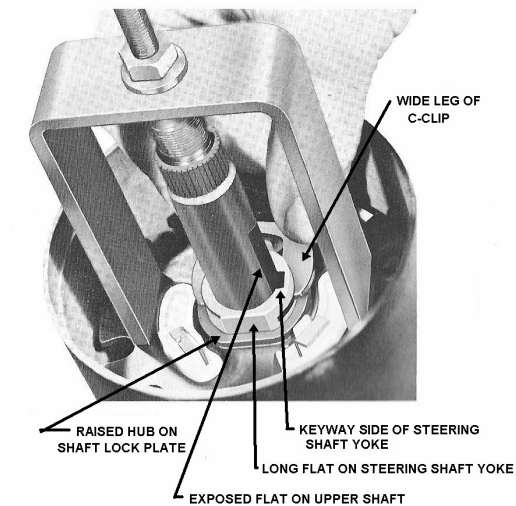
Fig. 3 C-Clip Installation
