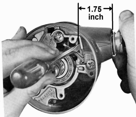
Fig. 1 Removing Lock Cylinder 1969 through Early 1979 T&T Steering Columns
