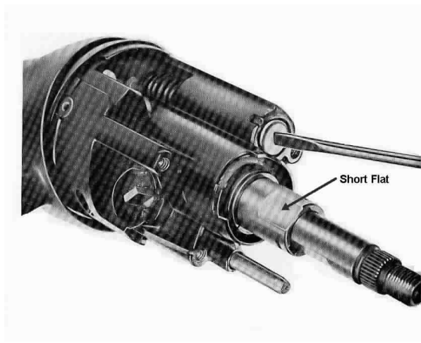
Fig. 2 Flats on Shaft Yoke
