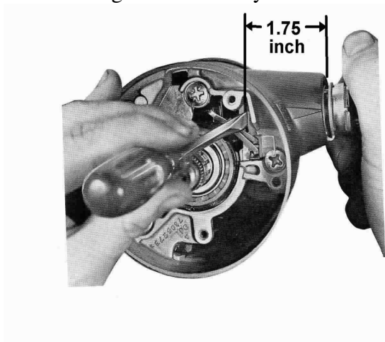
Fig. 1 Removing Lock Cylinder 1969 through Early 1979 T&T Steering Columns Removing Lock Cylinder (Continued)
