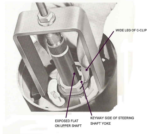
Fig. 3 C-Clip Installation
