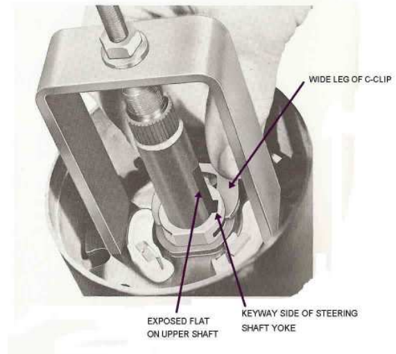
Fig. 3 C-Clip Installation
